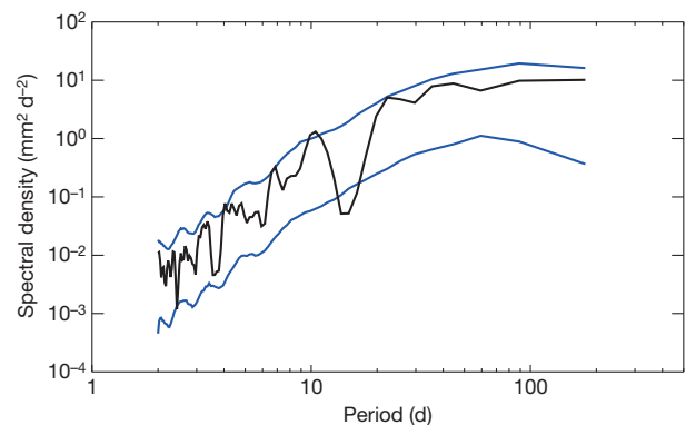
Figure 2 | Power spectra of daily river runoff for England and Wales autumns. Black line shows the spectrum for runoff synthesized from ERA-40 precipitation in all available autumns (1958–2001). Pair of blue lines marks the 5–95% confidence interval of the spectrum for runoff synthesized from all precipitation simulations in the A2000 climate.
