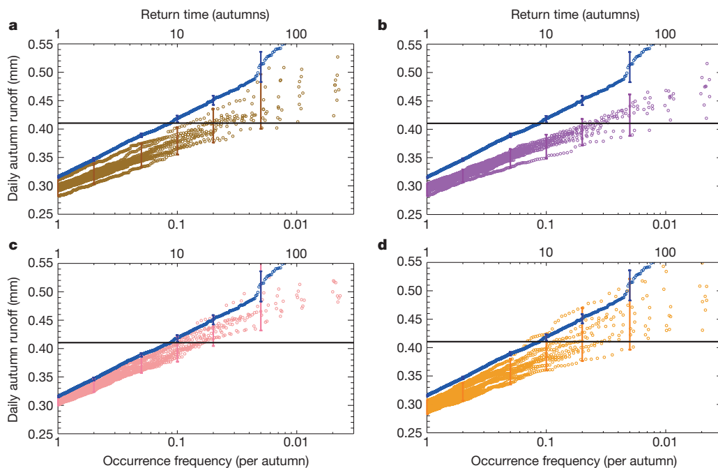
Figure 3 | Change in occurrence frequency of daily river runoff for England and Wales autumn 2000. a–d, Occurrence frequency curves of runoff (circles) synthesized from all precipitation simulations in A2000 and A2000N climates. Top axis of each panel is equivalent return time. Each panel shows identical A2000 runoff (blue). A2000N runoffs differ, being in climates generated using attributable SST warming estimates from HadCM3 (a; brown), GFDLR30 (b; purple), NCARPCM1 (c; pink) and MIROC3.2 (d; orange), with 10 curves corresponding to equiprobable amplitudes of warming. Bars represent 5–95% confidence intervals (see Methods). Horizontal line marks the highest autumn 2000 runoff synthesized from ERA-40 precipitation (0.41 mm).
